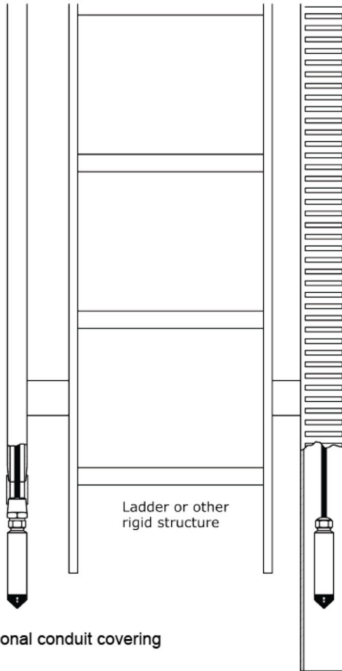
SNR-PP installed in customer supplied stilling well.
